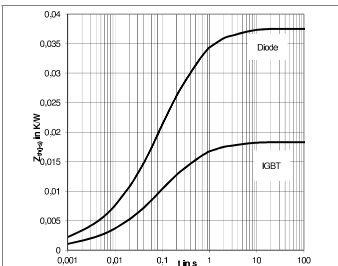
Fig. 5: Transient thermal impedance Z_{th(j-r)}
