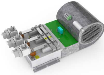
Diode Presspack stack
